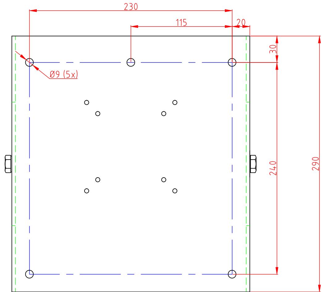
Equipment Platform
